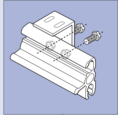
Side guide bracket
